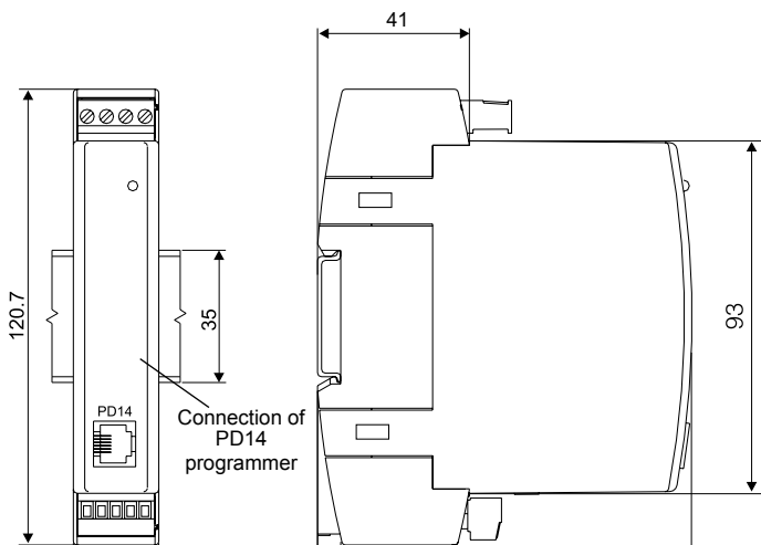
Fig 1. Dimensions and mounting of the transducer.
